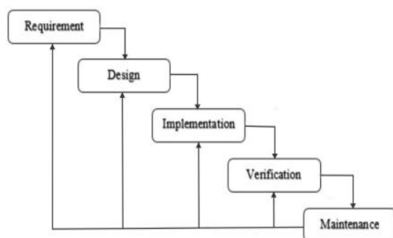
Gambar 2. Model Waterfall
